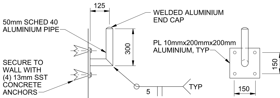
SINGLE PIPE MOUNT
