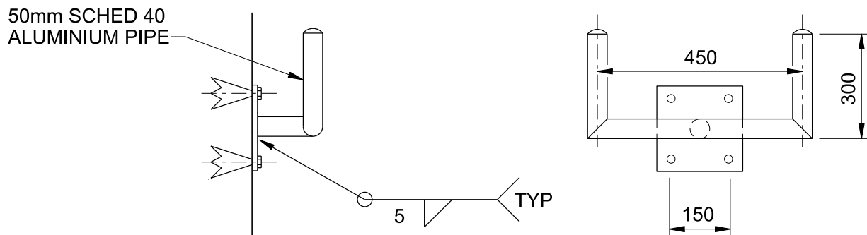
DUAL PIPE MOUNT
